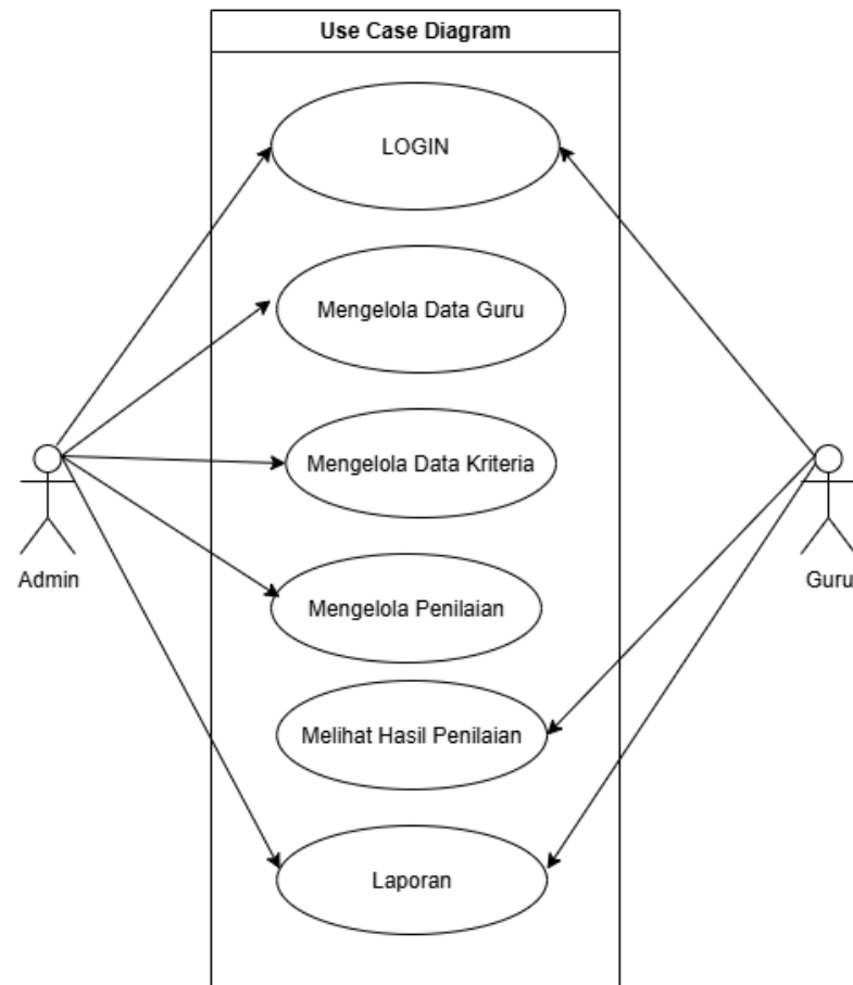
Gambar 4. 1 Use Case Diagram
